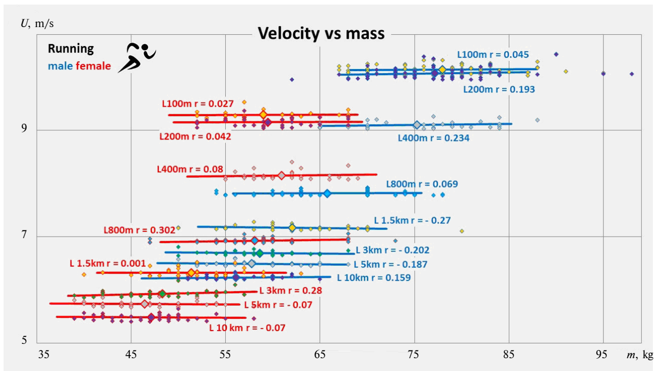
Figure 1: Running. The values of body mass and velocity. Small rhombuses are values for every athlete. Greater rhombuses are average values for every distance. The boundaries of rhombuses, corresponding linear regression lines and regression coefficients are blue for males and red for females
